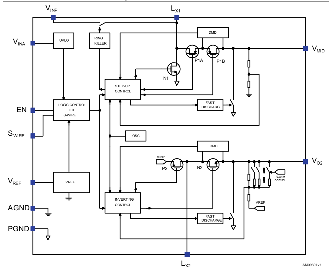
Figure 2. Block schematic
