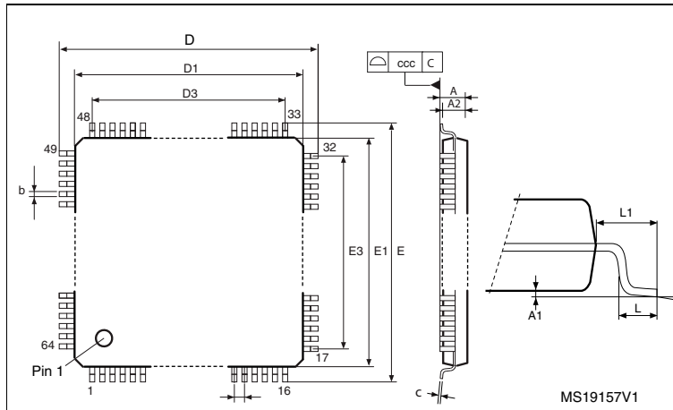
Figure 48. LQFP64 – 10 x 10 mm, 64 pin low-profile quad flat package outline (1)
