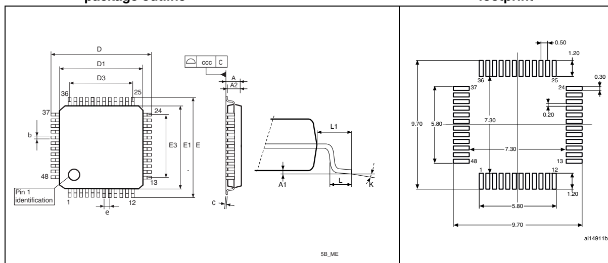
Figure 51. Recommended footprint (1)(2)
