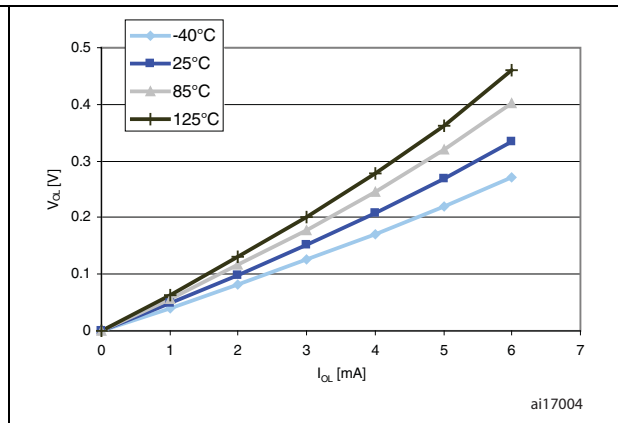
Figure 25. Typ. V_{OL} @ V_{DD} = 1.8 V (standard ports)
