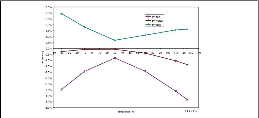
Figure 17. Typical HSI accuracy at VDD = 3 V vs temperature
