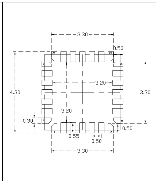
Figure 42. WFQFPN28 recommended footprint (1)(2)
