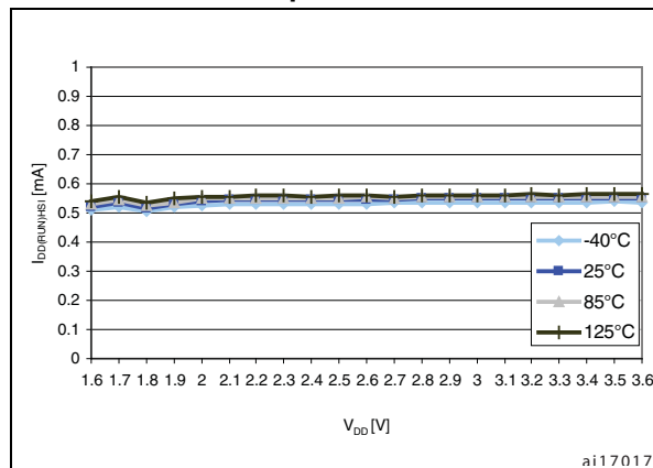
Figure 11. I_{DD(RUN)} vs. V_{DD} @ f_{CPU} = 2 MHz @4 temperatures
