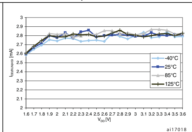
Figure 12. I_{DD(RUN)} vs. V_{DD} @ f_{CPU} = 16 MHz @4 temperatures
