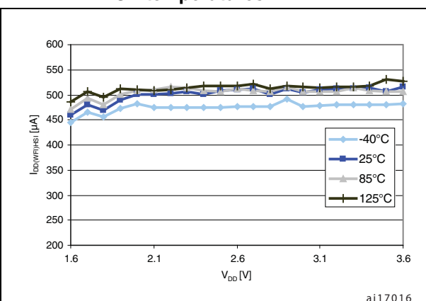
Figure 14. I_{DD(WAIT)} vs. V_{DD} @ f_{CPU} = 16\text{ MHz} @4 temperatures
