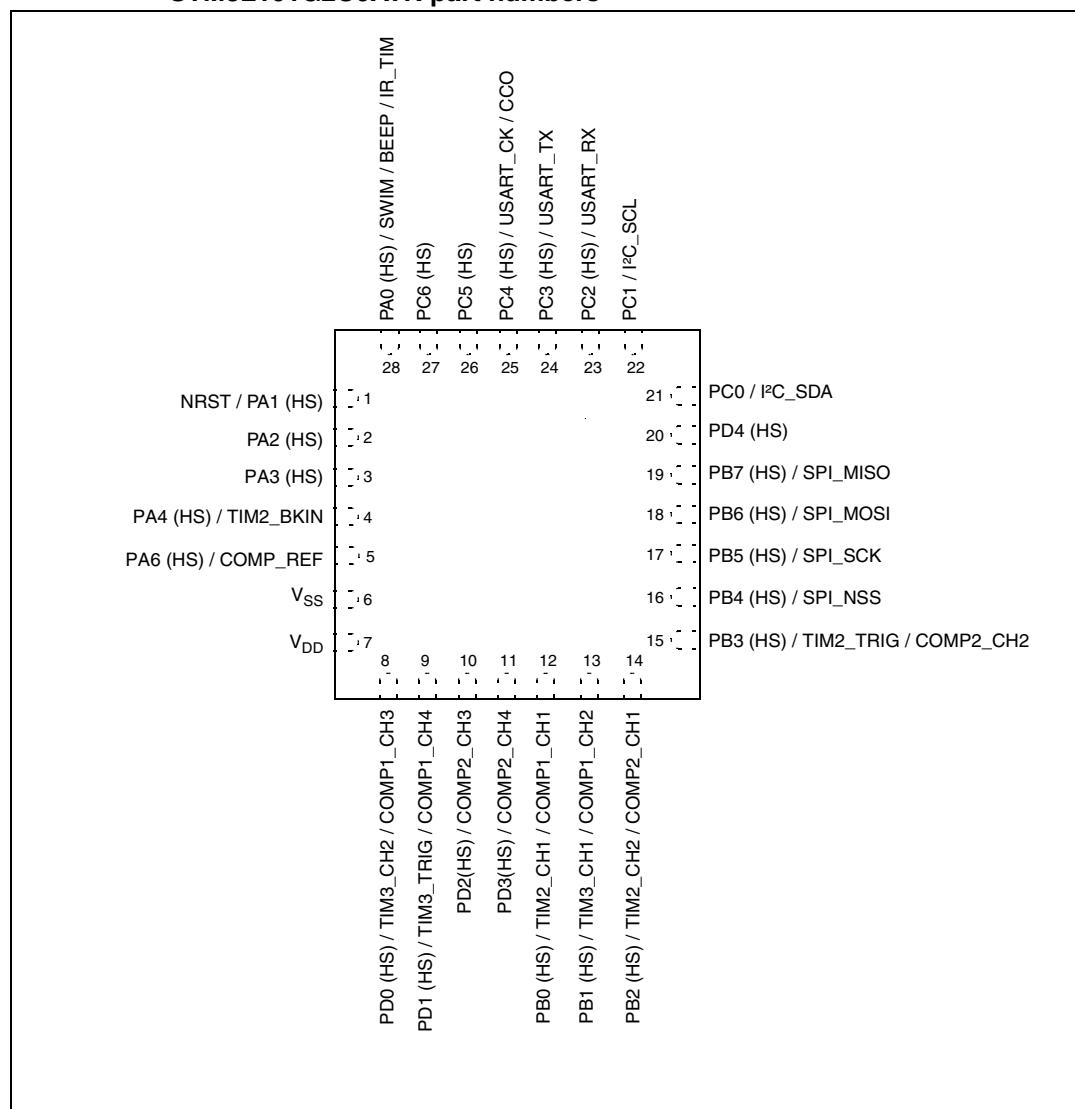
Figure 6. 28-pin WFQFPN package pinout for STM8L101G3U6ATR and STM8L101G2U6ATR part numbers
