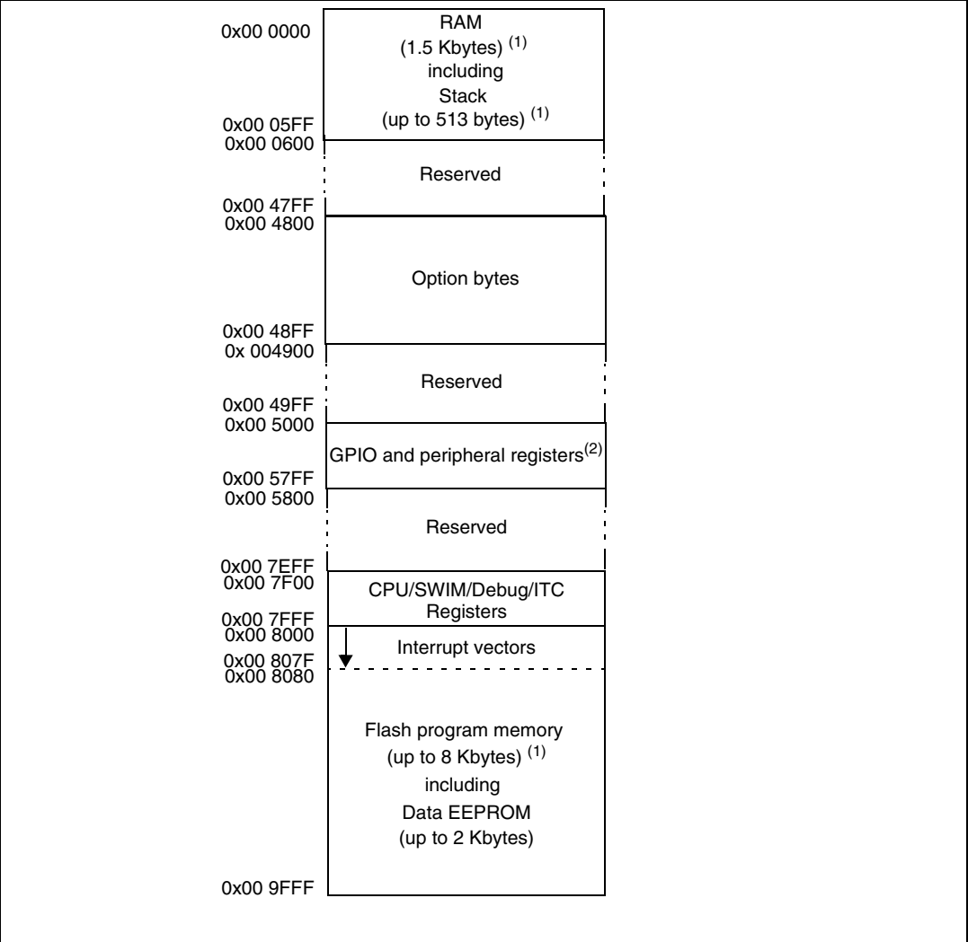
Figure 8. Memory map
