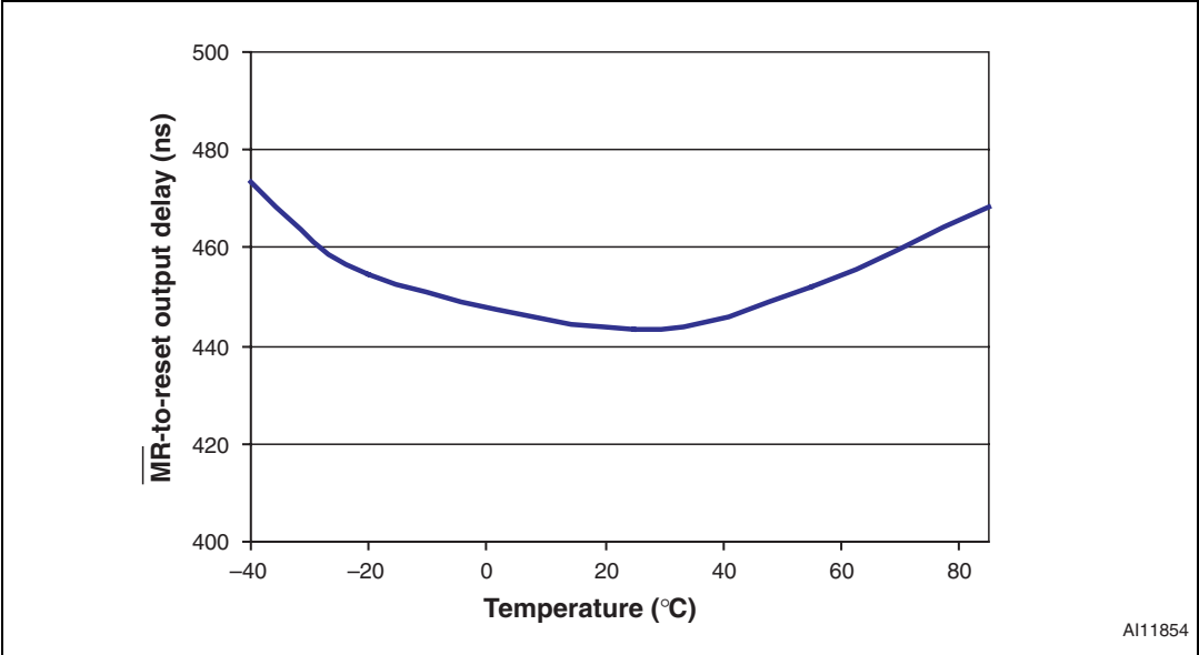
Figure 24. \overline{\text{MR}} -to-reset output delay vs. temperature ( V_{\text{CC1}} = 3.6\text{V} )
