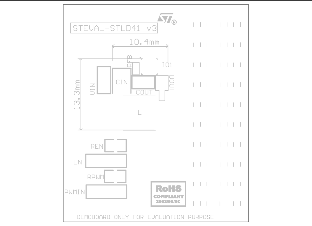
Figure 6. Top overlay
