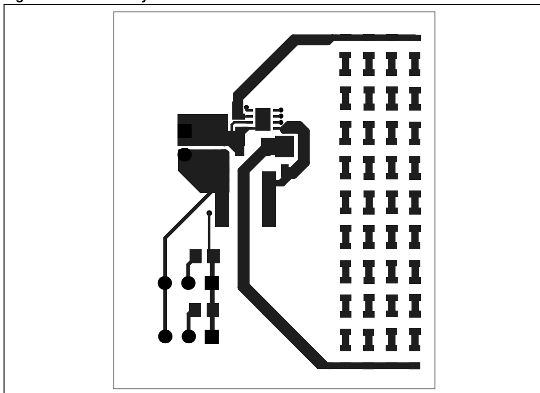
Figure 5. Bottom layer
