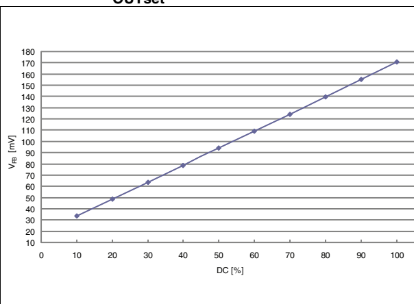
Figure 12. V_{FB} vs. PWM 25 kHz, V_{IN} = 5.5 V, I_{OUTset} = 120 mA
