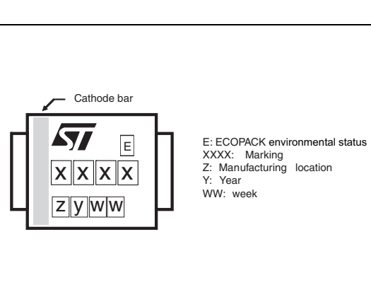
Figure 12. Marking layout
