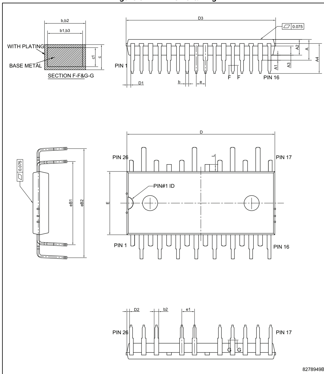
Figure 9. NDIP-26L drawing
