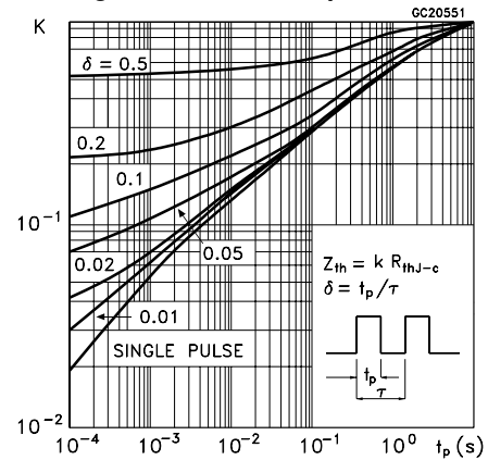
Figure 3: Thermal impedance
