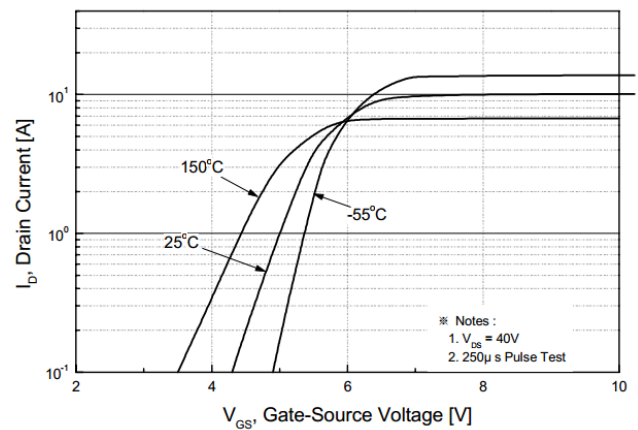
Figure 2. Transfer Characteristics
