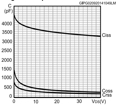
Figure 8: Capacitance variation
