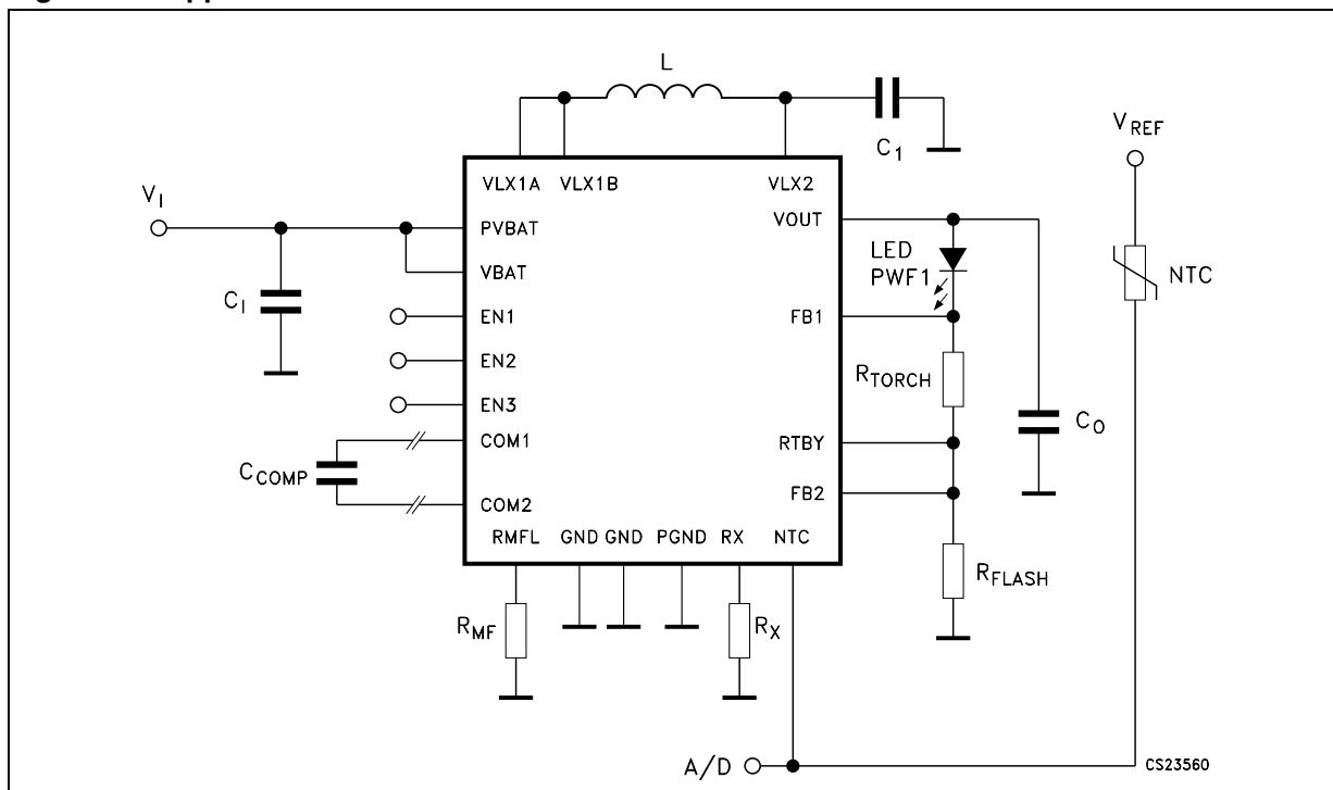
Figure 1. Application circuit
