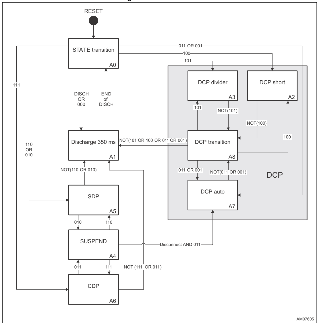
Figure 5. State machine
