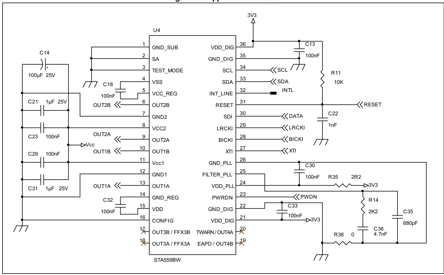
Figure 19. Applications circuit
