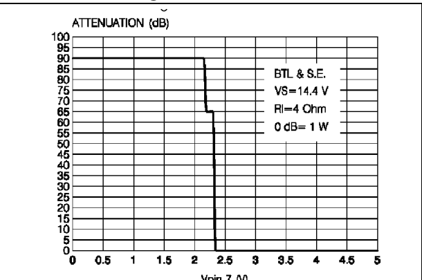
Figure 22. Standby attenuation vs threshold voltage
