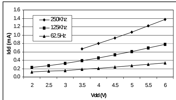
Figure 64. Typical I_{DD} in SLOW vs. f_{CPU}
