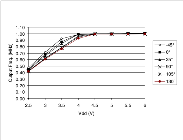
Figure 57. RC Osc Freq vs V_{DD} (Calibrated with RCCR0: 5V @ 25^{\circ}\text{C} )
