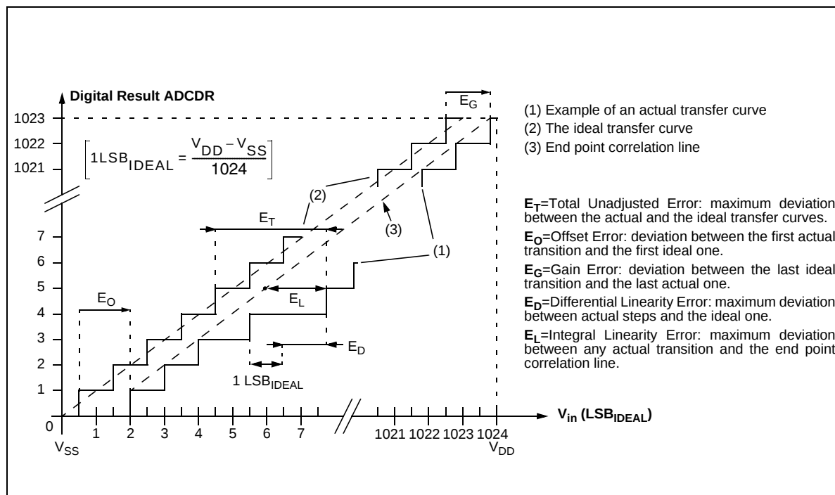
Figure 92. ADC Accuracy Characteristics with amplifier disabled
