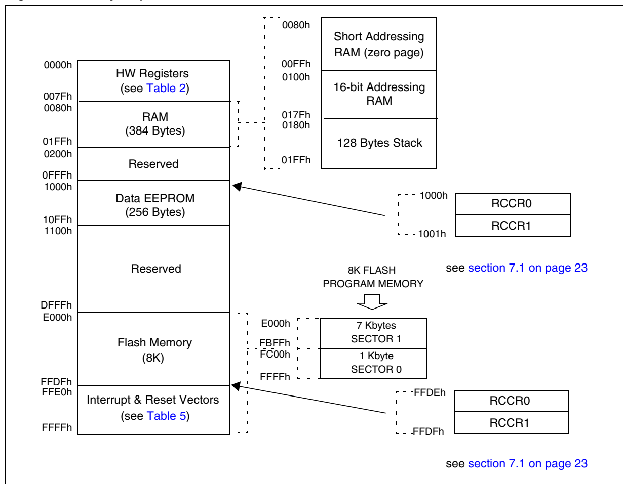
Figure 3. Memory Map
