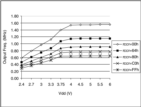
Figure 59. RC Osc Freq vs V_{DD} and RCCR Value
