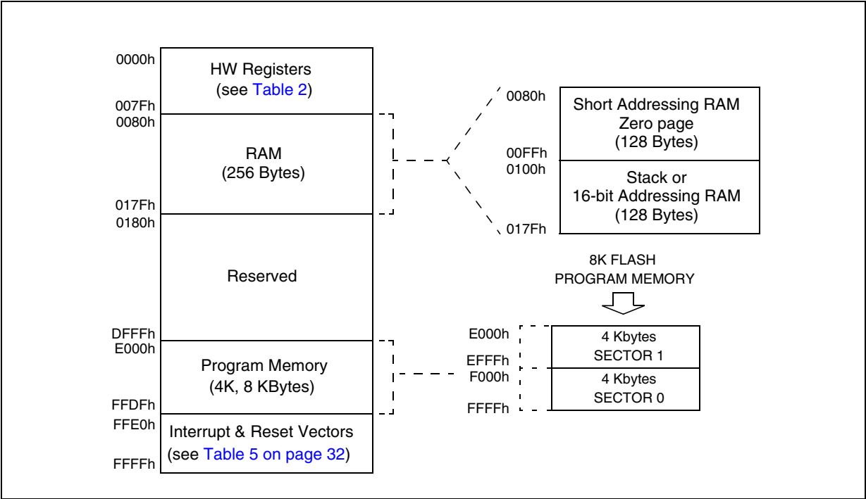
Figure 5. Memory Map
