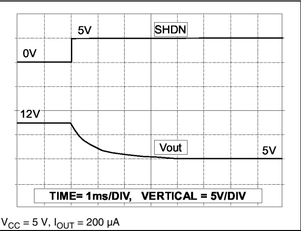
Figure 14. Entering shutdown
