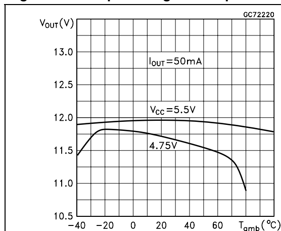
Figure 3. Output voltage vs temperature
