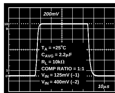
Figure 9. Large Signal Transient Response
