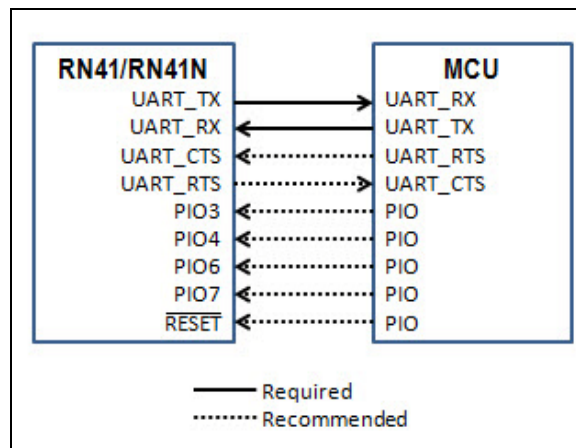
FIGURE 1-1: RN41/RN41N TO MCU INTERFACE
