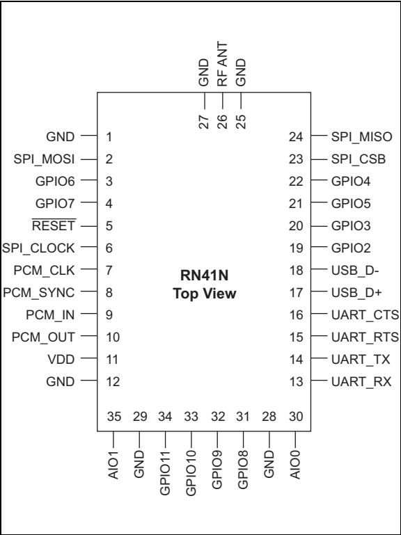
FIGURE 1-5: RN41N PIN DIAGRAM
