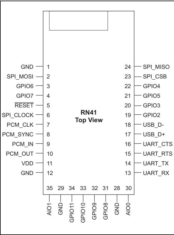
FIGURE 1-4: RN41 PIN DIAGRAM
