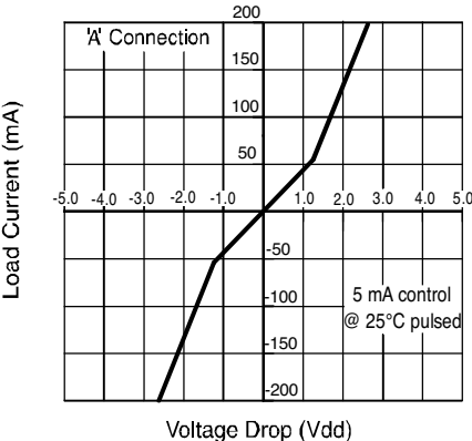
Figure 3. Linearity Characteristics
