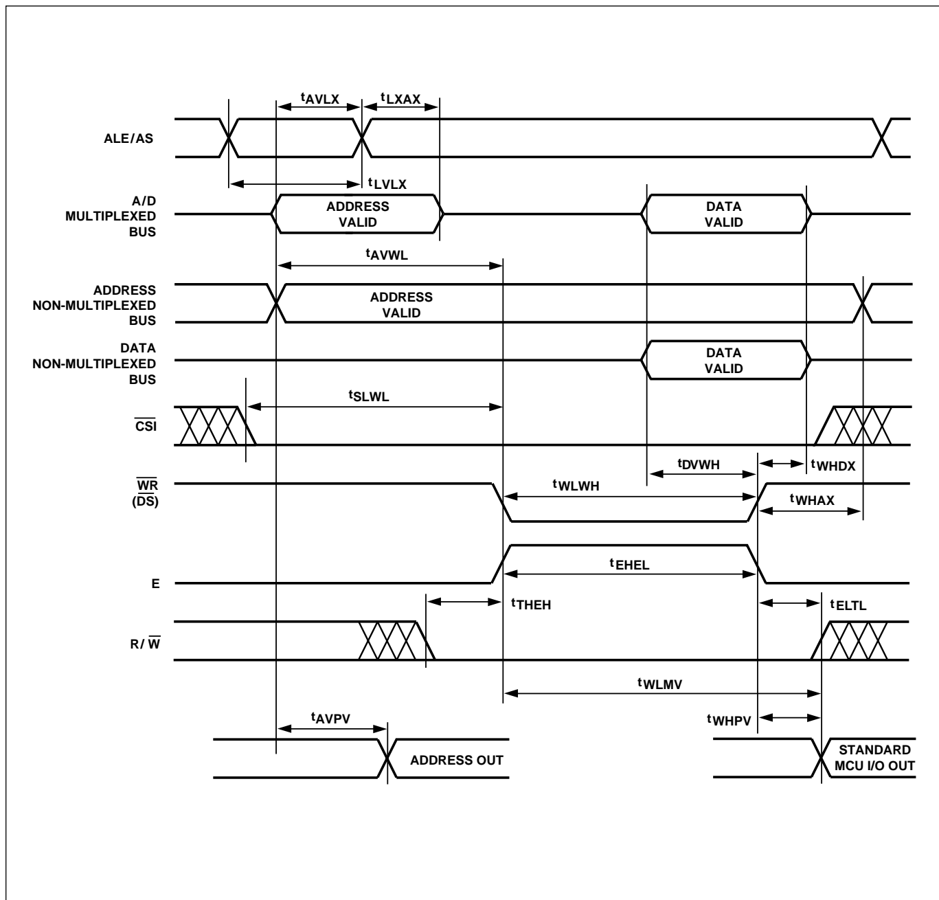
Figure 34. Write Timing
