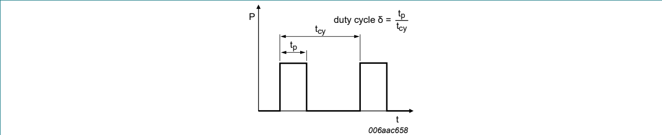
Fig. 14. Duty cycle definition
