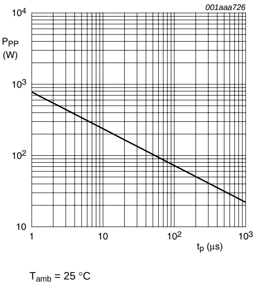
Fig 4. Peak pulse power as a function of exponential pulse duration; typical values
