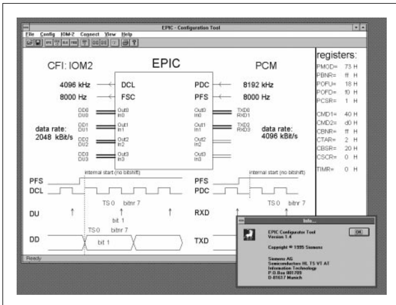
Figure 107 EPIC® Configuration Tool: Screen Shot
