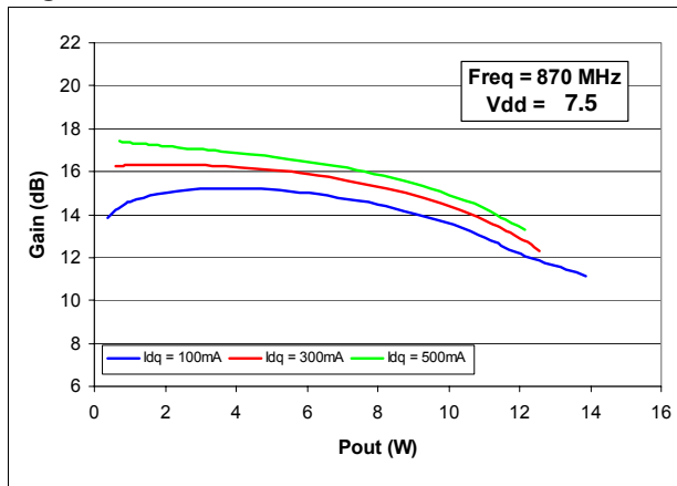
Figure 11. Gain vs Pout &amp; Bias current
