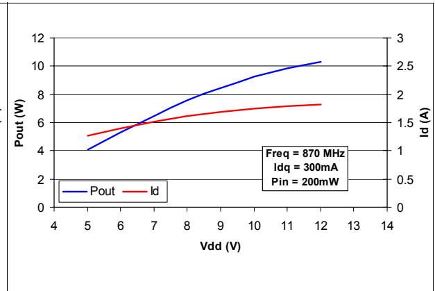
Figure 10. Pout &amp; id vs supply voltage
