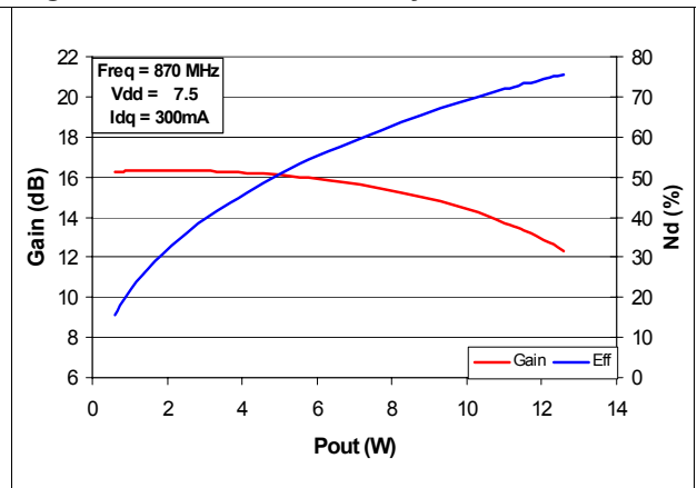
Figure 12. Gain &amp; efficiency vs Pout
