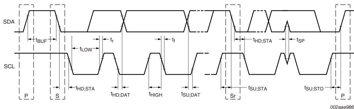
Fig 12. Timing diagram for serial interface
