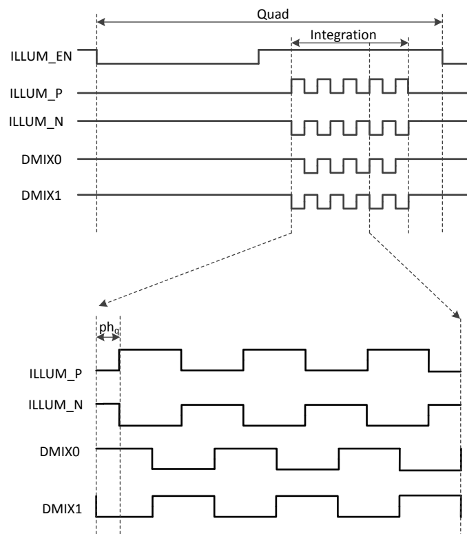
Figure 3. Timing Diagram
