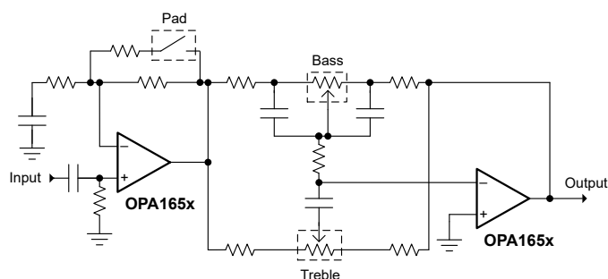
Active Baxandall Tone Control
