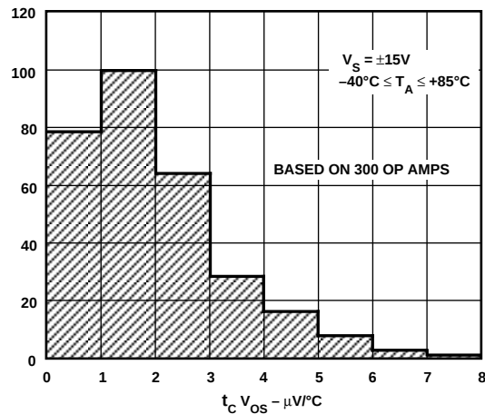
Figure 1. Input Offset Voltage Drift Distribution @ ±15 V
