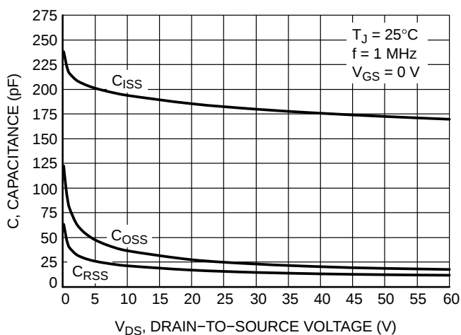
Figure 9. Capacitance Variation
