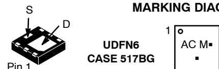
P–Channel MOSFET
