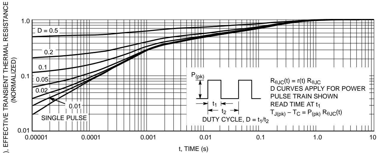
Figure 13. Thermal Response
