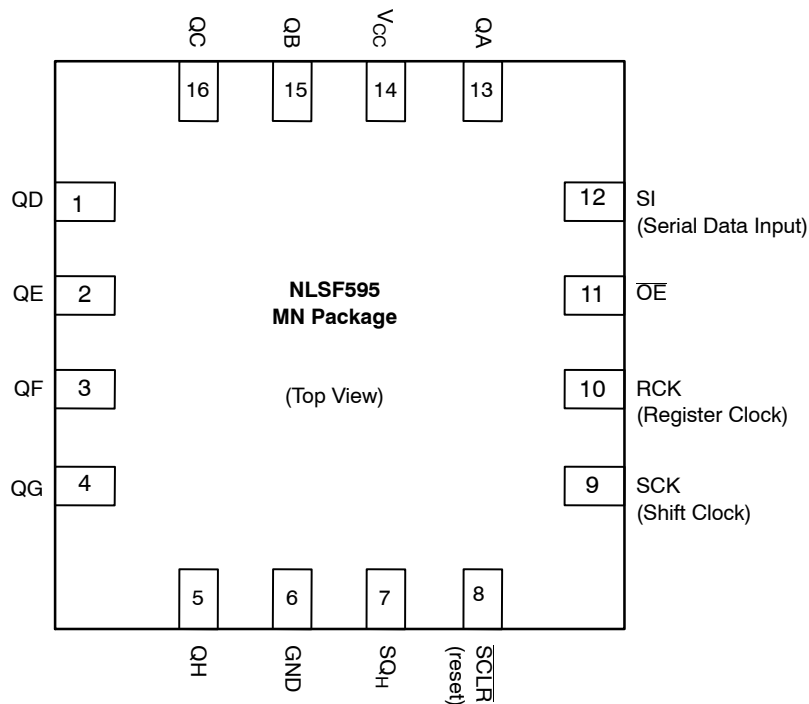
Figure 3. Pin Assignment (QFN-16)
