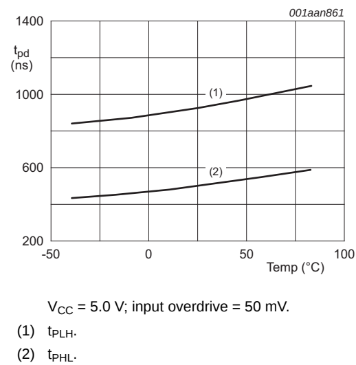
Fig 13. Propagation delay versus temperature
