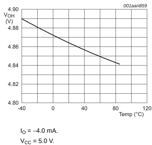
Fig 11. HIGH-level output voltage versus temperature
