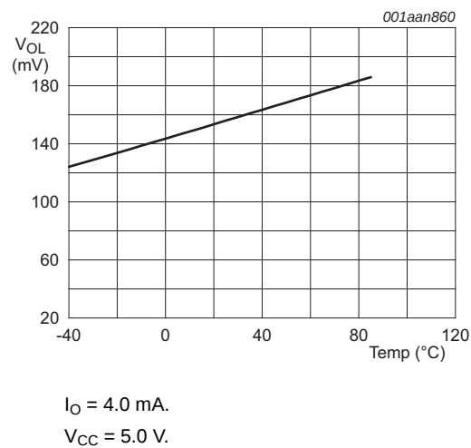
Fig 12. LOW-level output voltage versus temperature
