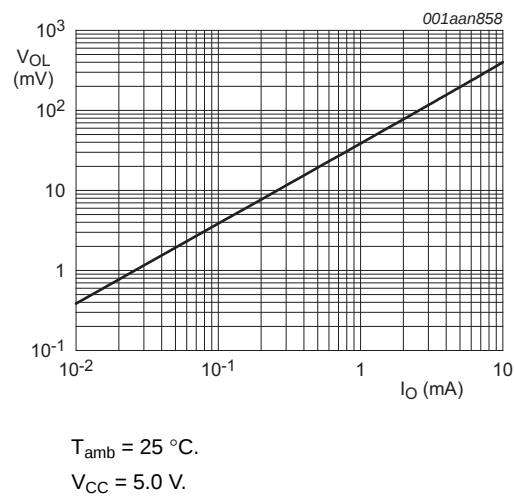
Fig 10. LOW-level output voltage versus output current
