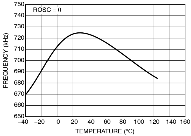
Figure 27. Maximum Switching Frequency vs. Temperature
