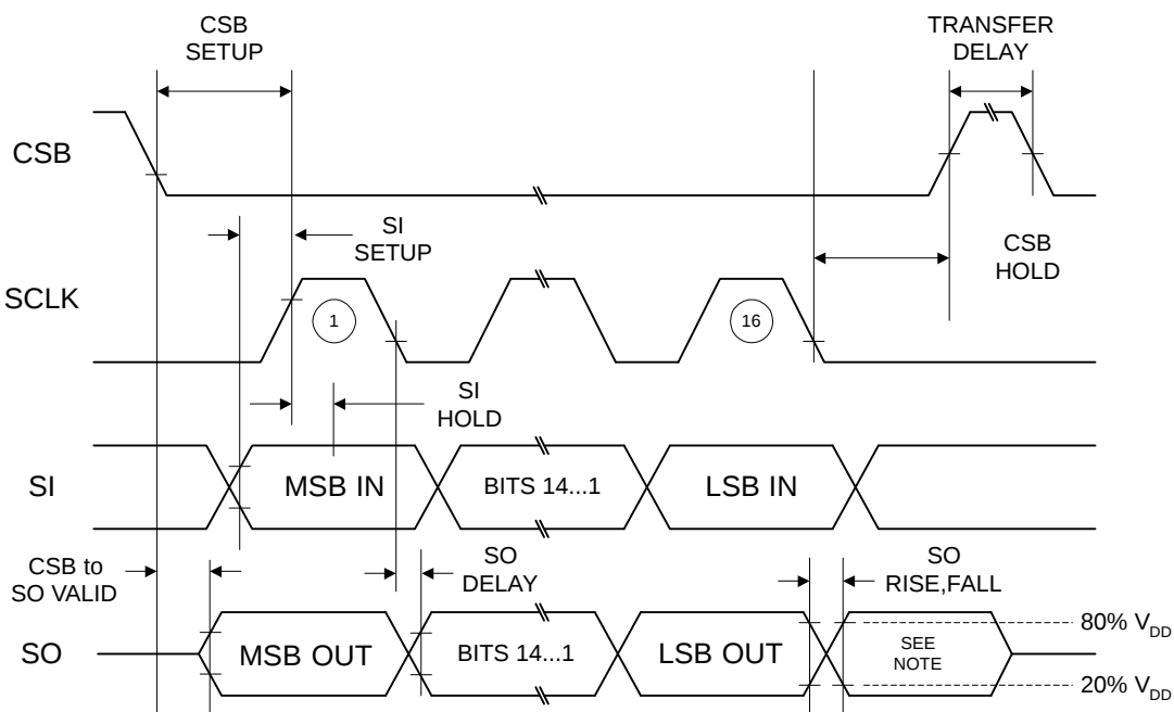
Figure 9. SPI Timing Diagram
