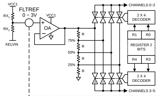
Figure 13. Shorted Load Reference Generator
