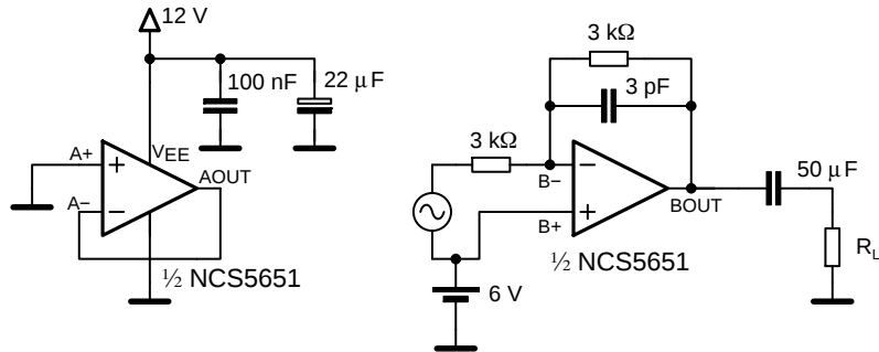
Figure 5. Test Circuit for Figures 3 and 4
