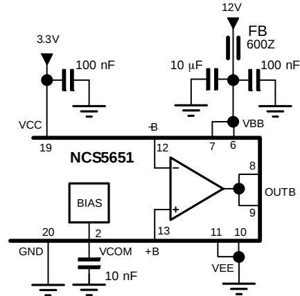
Figure 9. Decoupling Capacitors
