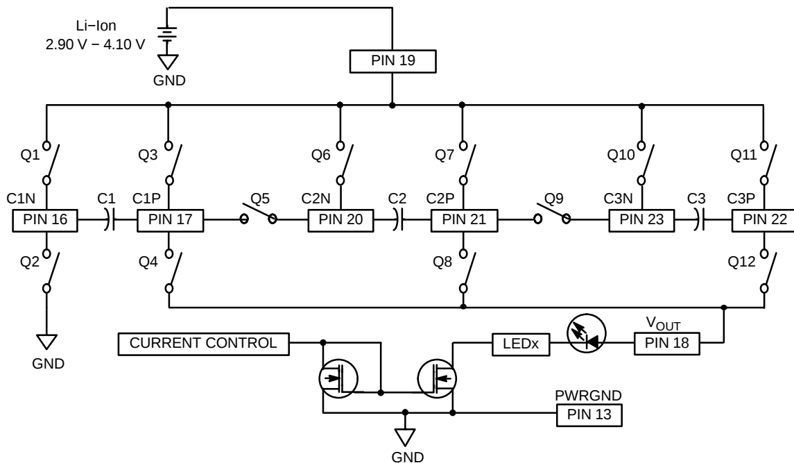
Figure 3. Basic DC-DC NCP5608 Converter Structure
