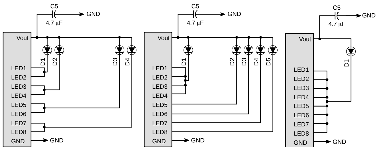
Figure 16. Examples of Possible LED Arrangements
