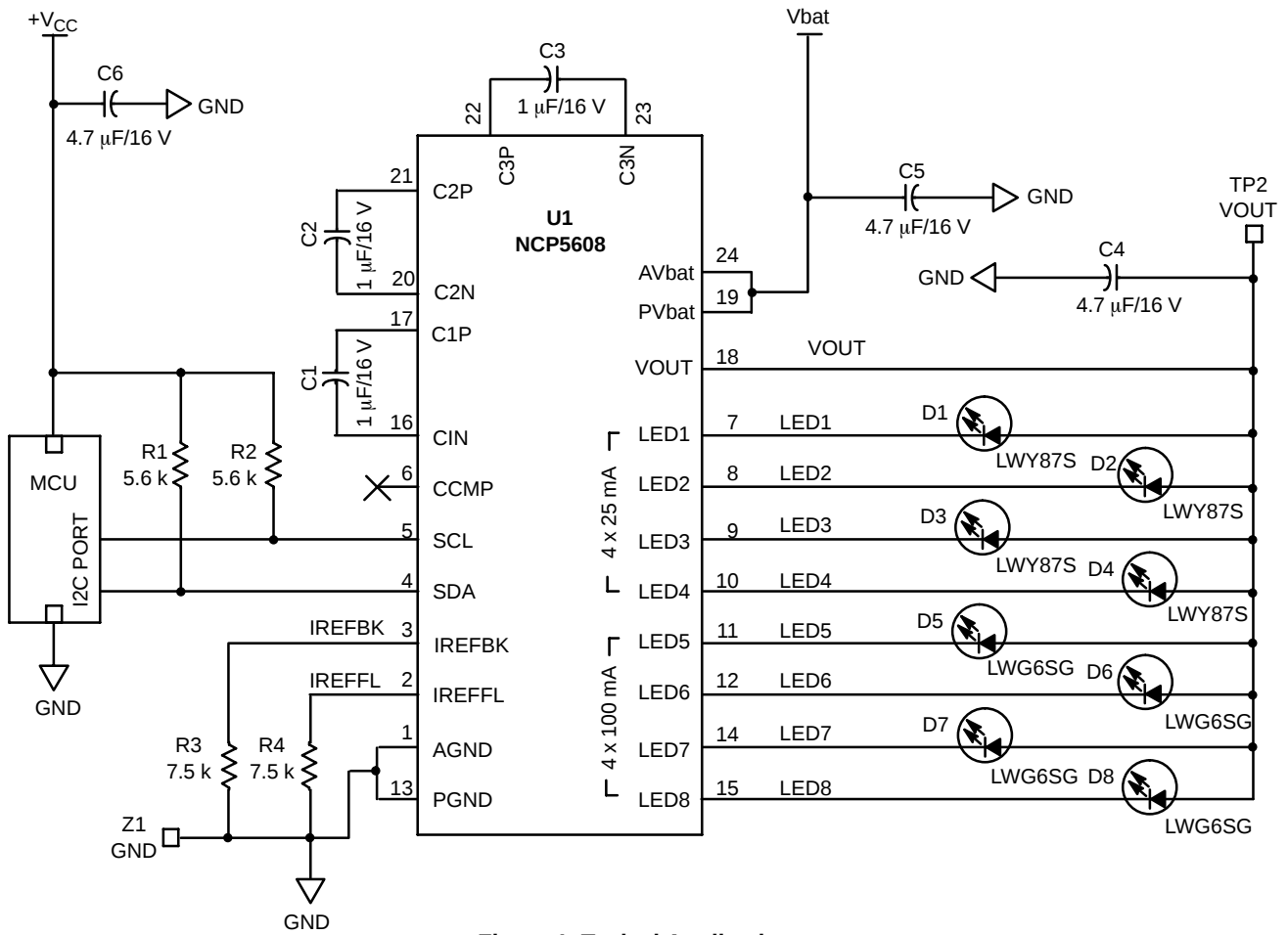
Figure 1. Typical Application
