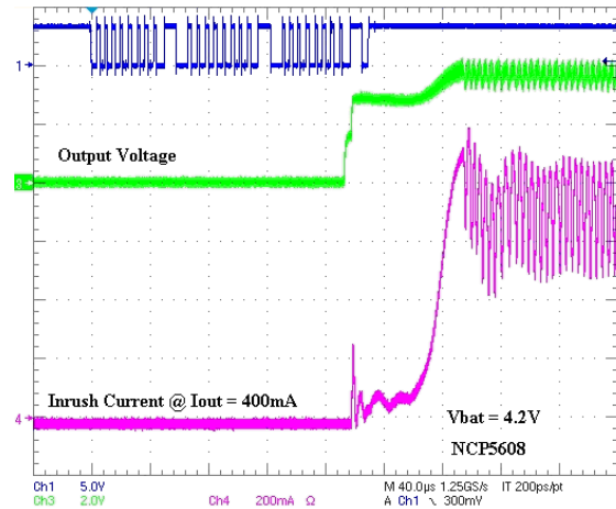
Figure 13. Typical Powerup Response
