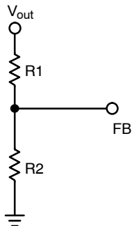
Figure 25. Output divider
