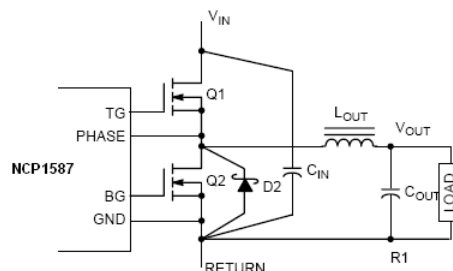
Figure 12. Components to be Considered for Layout Specifications
