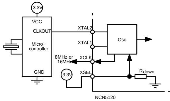
Figure 19. External Clock Generator
