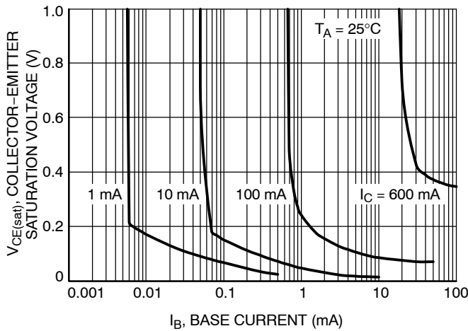
Figure 17. Saturation Region
