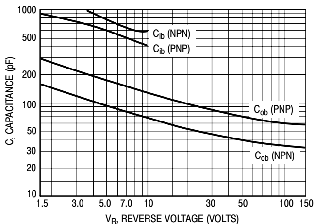
Figure 5. Capacitances
