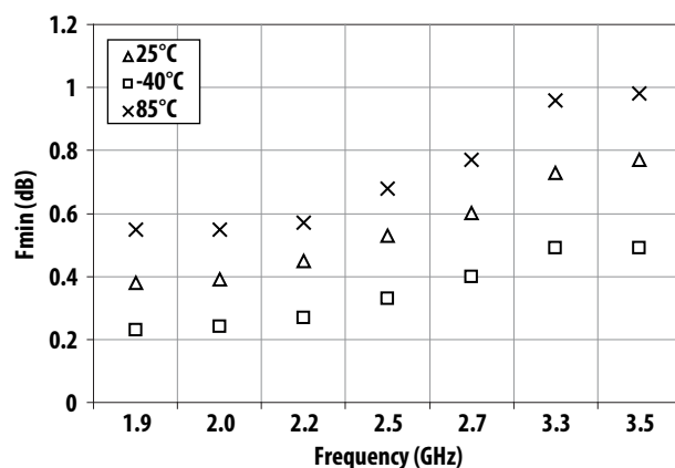
Figure 18. Fmin vs Frequency and Temperature for Optimum OIP3 and Fmin at 5V 55mA
