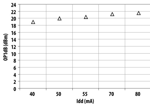
Figure 14. OP1dB vs Idd at 5V Tuned for Optimum OIP3 and Fmin at 2GHz.
