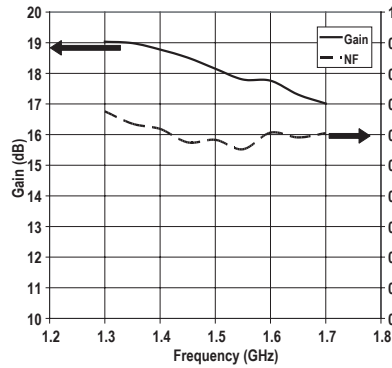
Figure 23. Gain and NF Vs Frequency
