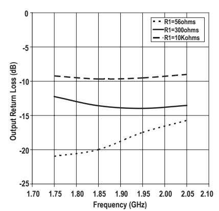
Figure 22. Output Return Loss vs Frequency and R1
