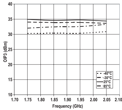
Figure 14. OIP3 vs Frequency and Temperature
