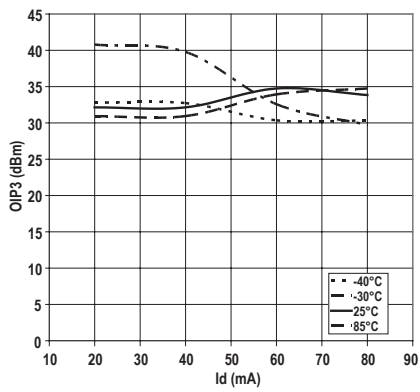
Figure 17. OIP3 vs Id and Temperature
