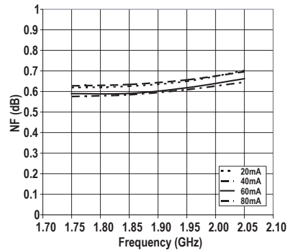
Figure 6. NF Vs Frequency and I_d
