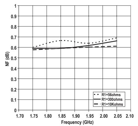
Figure 19. NF vs Frequency and R1
