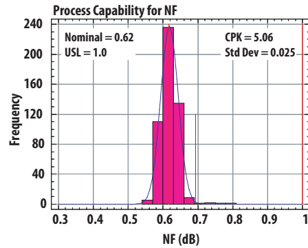
Figure 2. NF distribution at 57mA
