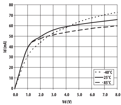
Figure 11. I_d Vs V_d and Temperature
