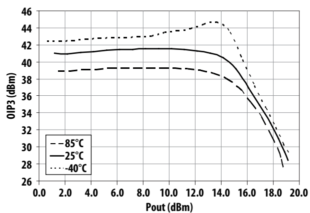
Figure 14. OIP3 vs Output Power and Temperature at 450MHz
