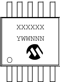
10-Lead MSOP (MCP655)
