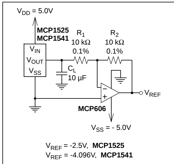
FIGURE 4-3: Negative Voltage Reference.
