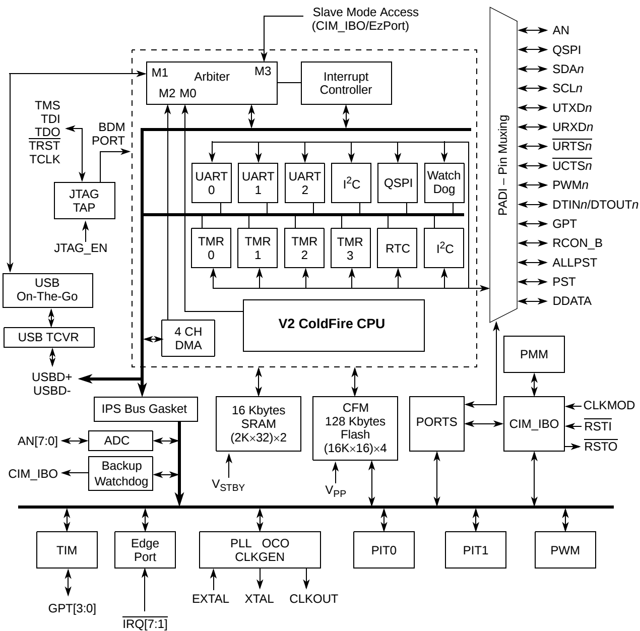
Figure 1. MCF52211 Block Diagram
