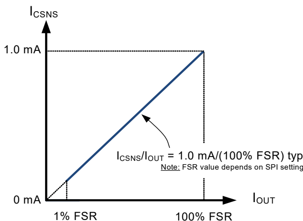
Figure 25. Output current sensing
